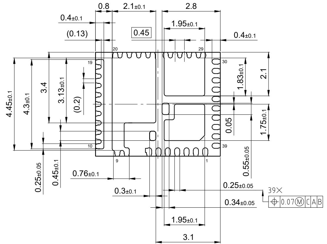
Bottom view
